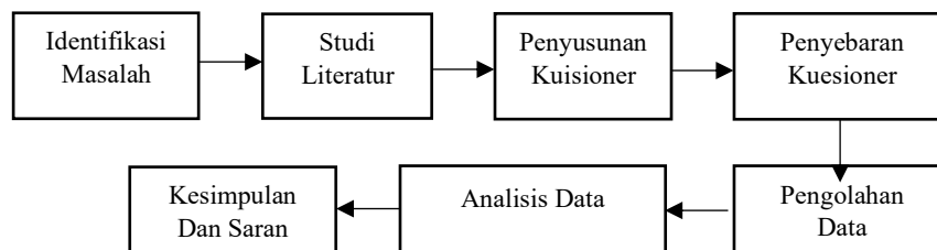
Gambar 3.1 Alur Penelitian
