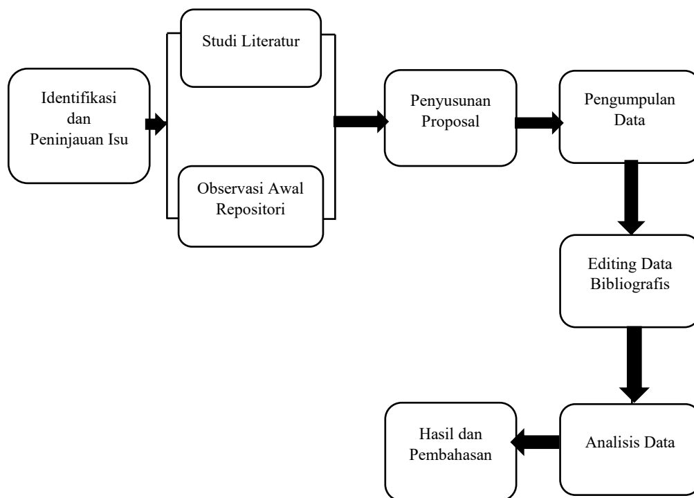
Gambar 3.1 Alur Penelitian
