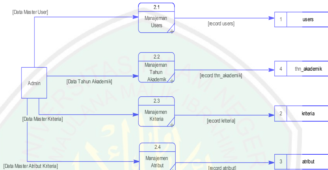
Gambar 3.7 DFD level 2 proses 2 olah master users
