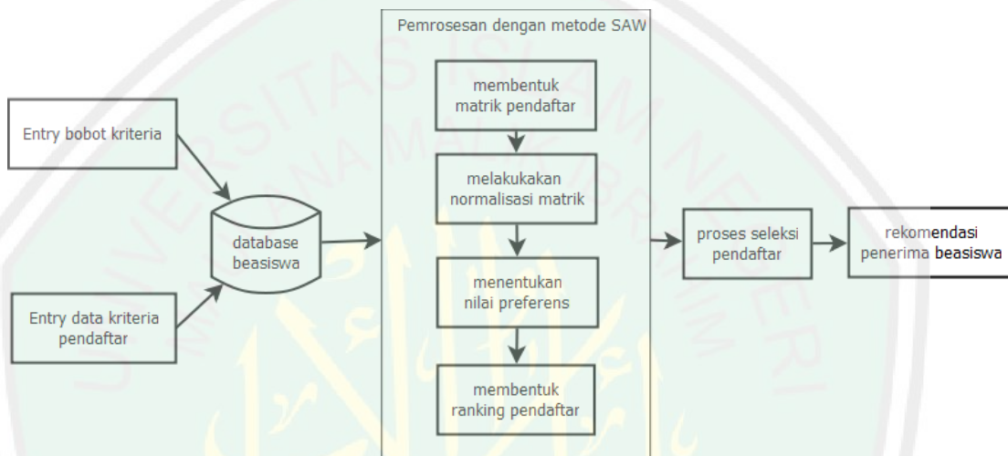
Gambar 3.3 Diagram Alur Sistem
