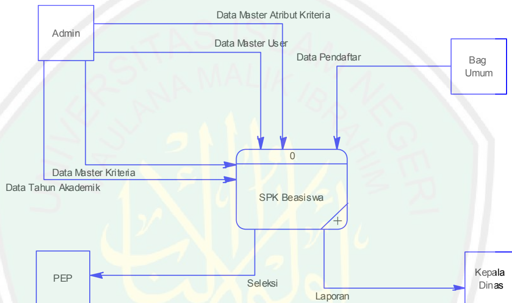
Gambar 3.5 Diagram konteks
