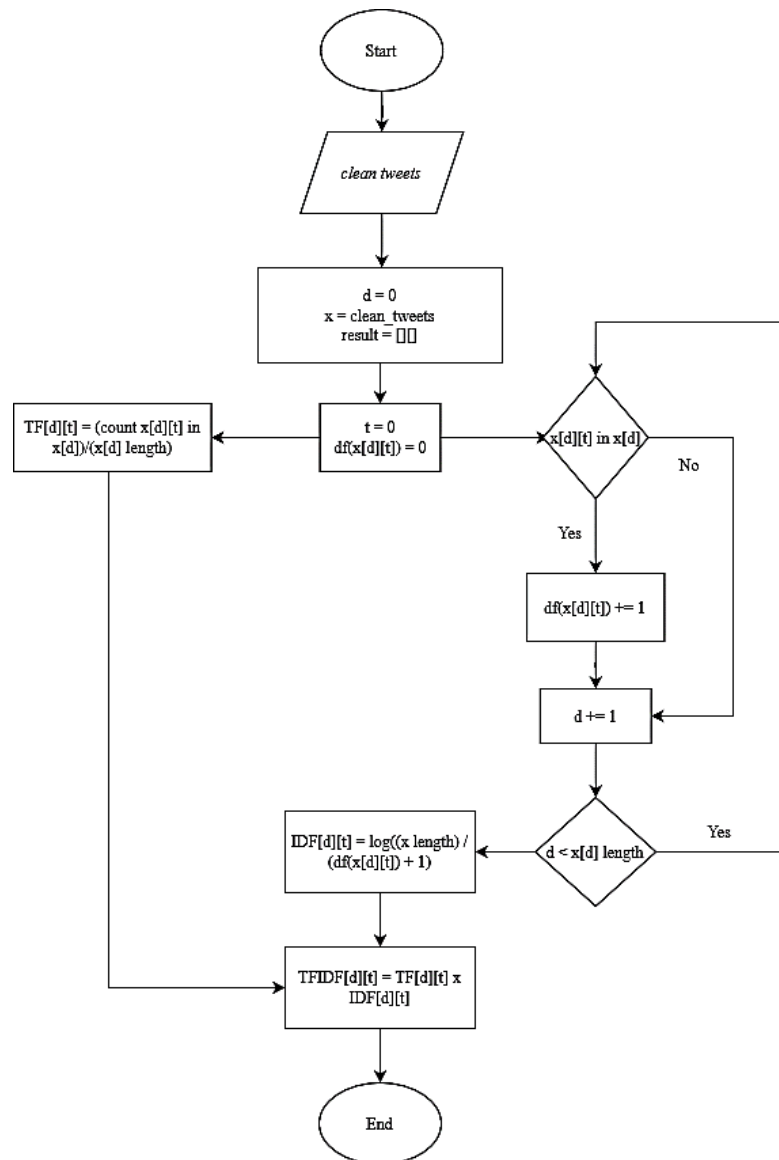
Gambar 3. 6 Flowchart TF-IDF
