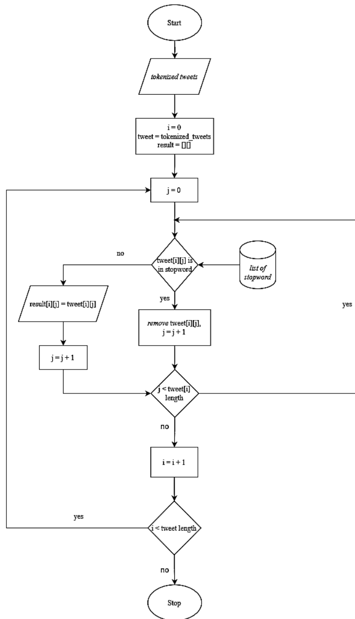
Gambar 3. 4 Flowchart stopwords removal
