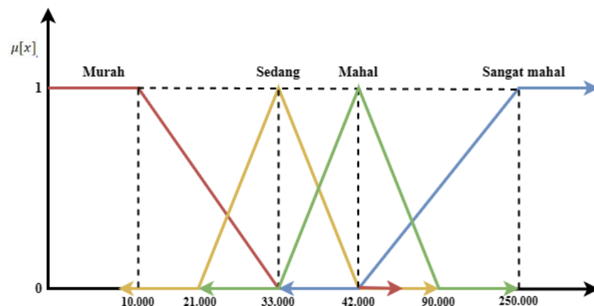
Gambar 4.1. Himpunan Fuzzy Variabel Harga
