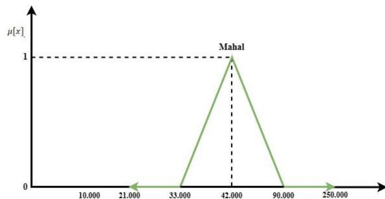
Gambar 4.4. Perhitungan Himpunan Fuzzy Harga Kain Mahal
