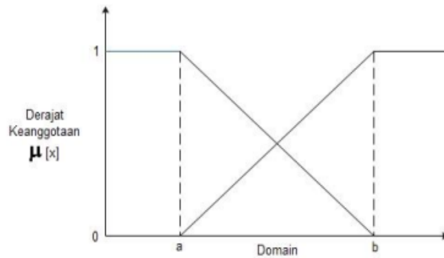
Gambar 2.4. Representasi Kurva Linear Bahu
