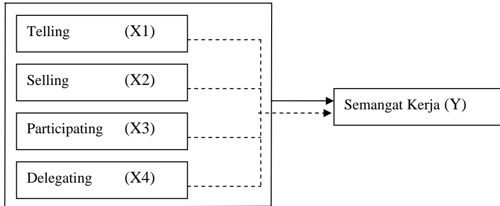
Gambar. 2.4 Model Hipotesis
