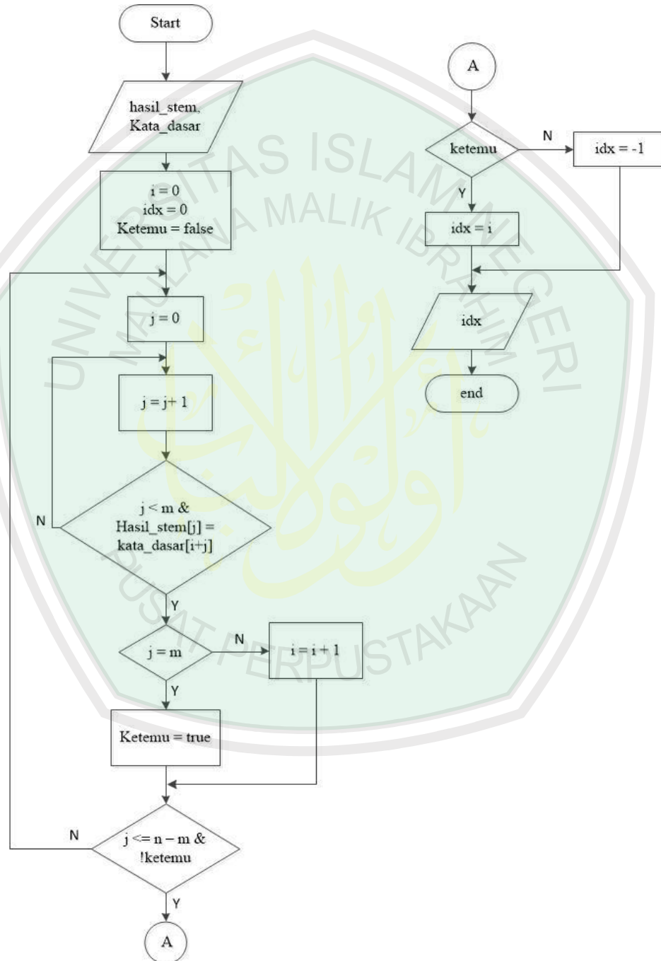
Gambar 3.3. flowchart diagram proses String Matching
