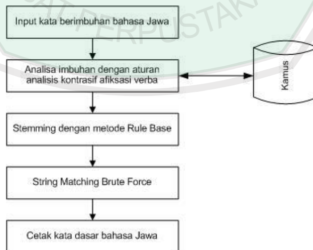
Gambar 3.1. Blok diagram proses algoritma stemming
