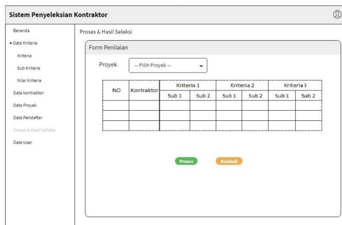
Gambar 3. 20 Halaman Proses Nilai
