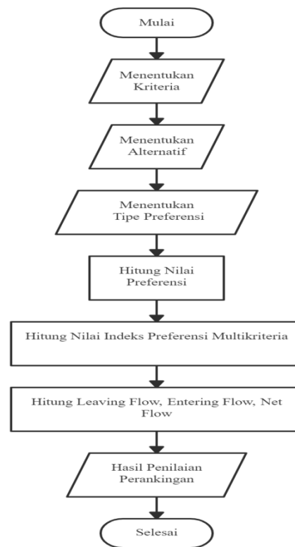
Gambar 3. 2 Flowchart Metode Promethee
