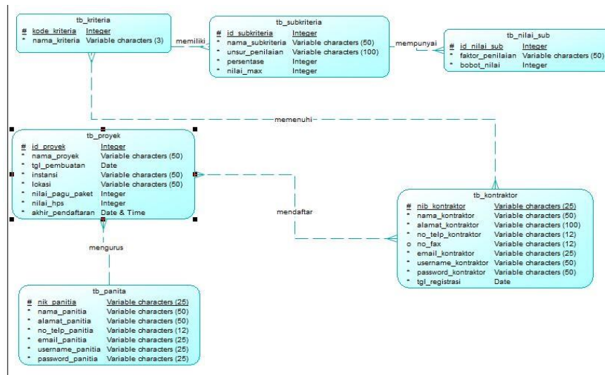
Gambar 3. 4 Conceptual Data Model
