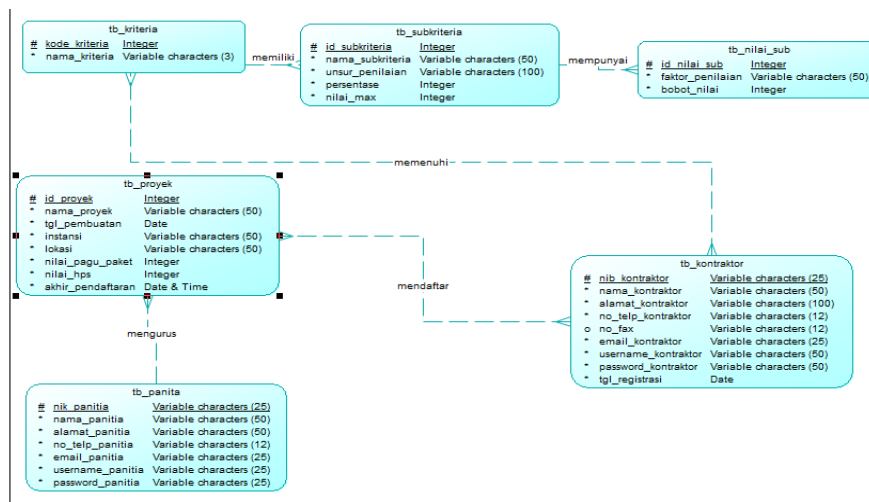
Gambar 3. 5 Physical Data Model
