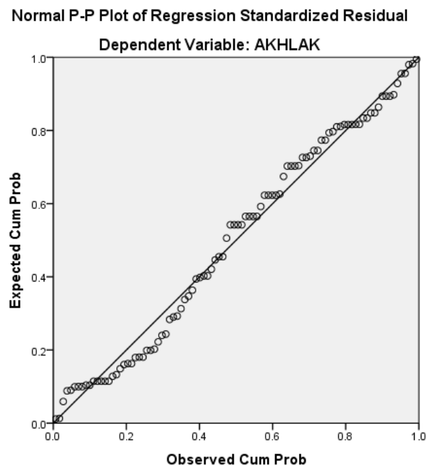
Gambar 4.1 Output Uji Normalitas metode Normal Probability Plots .
