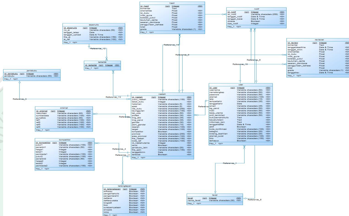
Gambar 3. 23 Conceptual Data Model
