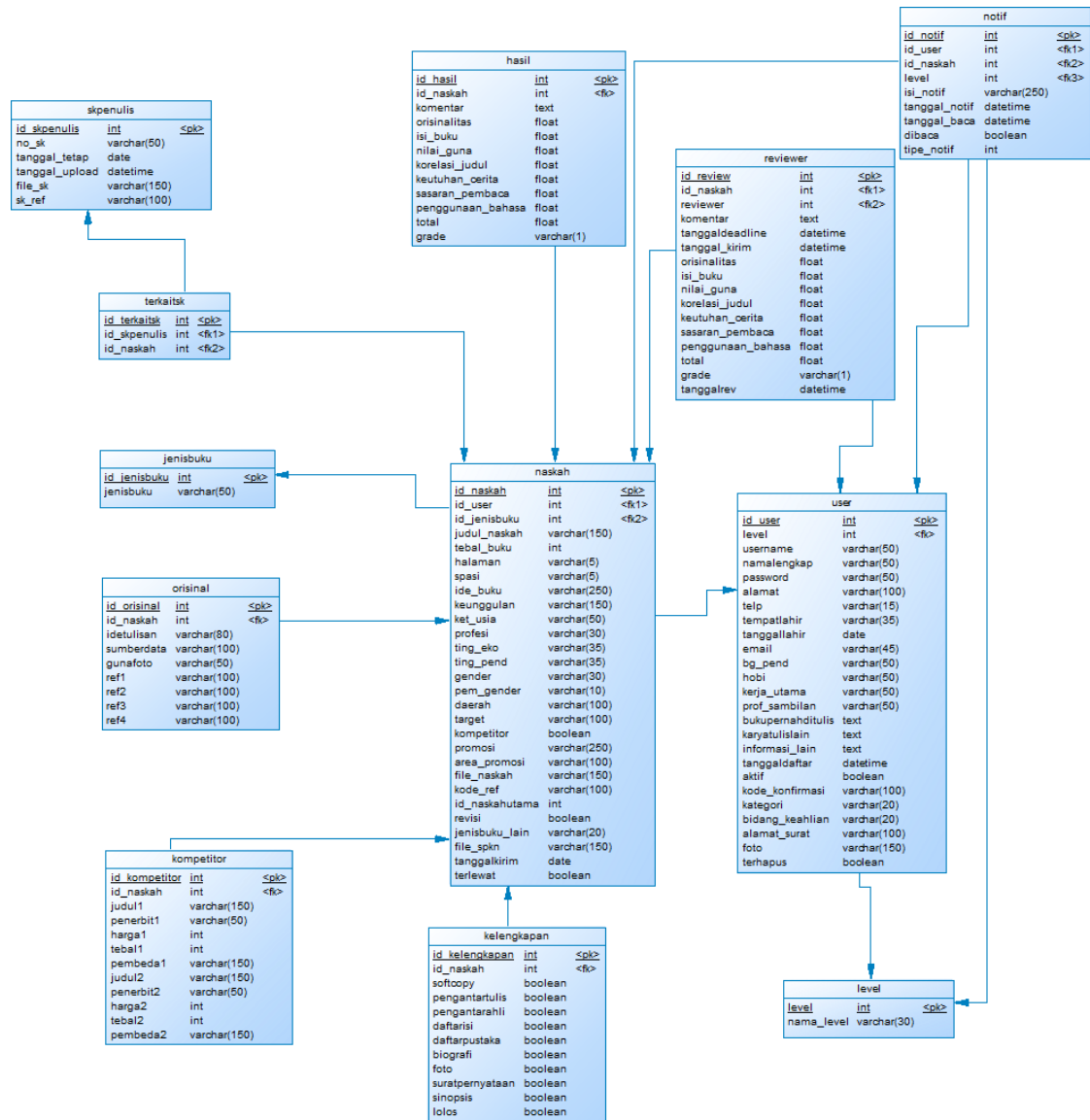
Gambar 3. 24 Physical Data Model
