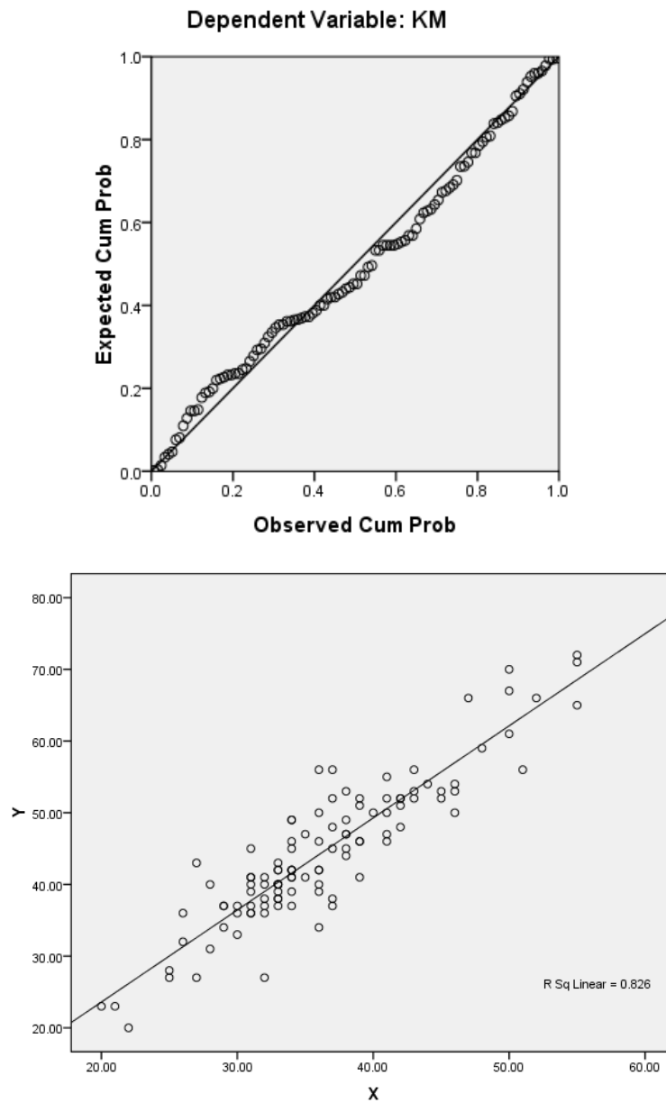
Normal P-P Plot of Regression Standardized Residual
