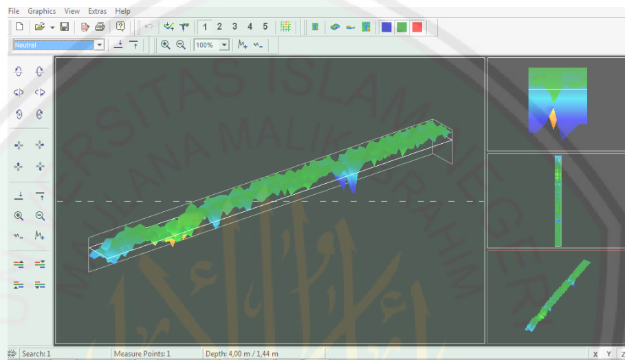
Gambar 4.13 Penampang 3D lintasan 3
